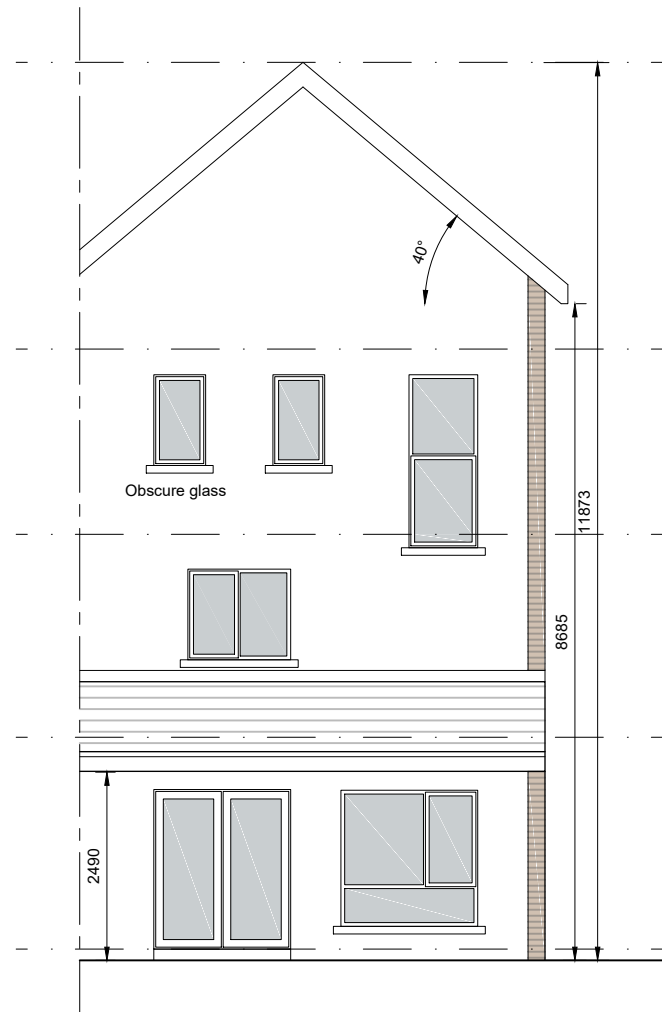
REAR ELEVATION
